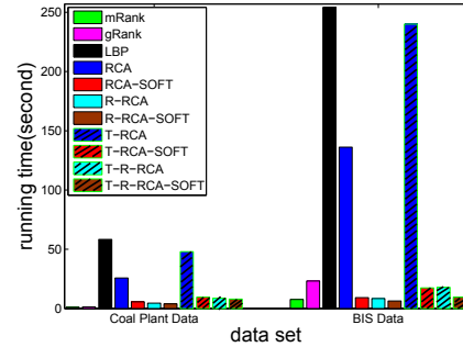
Figure 10: Running time on real data sets.
